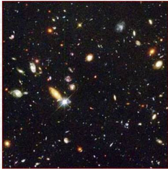
The Hubble Telescope "Deep Field"
